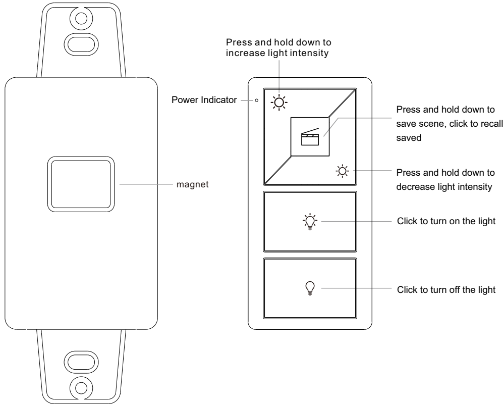
Bracket
